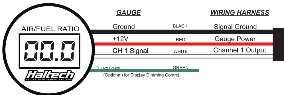
Figure 10 - Haltech Air/Fuel Ratio Digital Display Gauge
