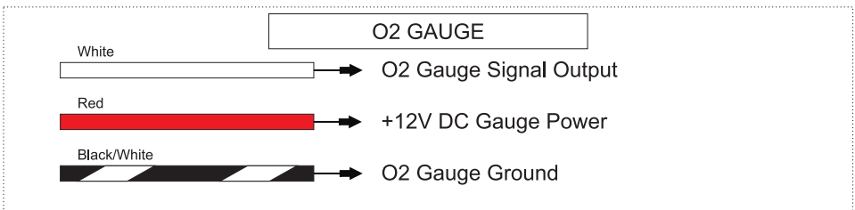
Figure 8 - In Cabin Harness Wiring
